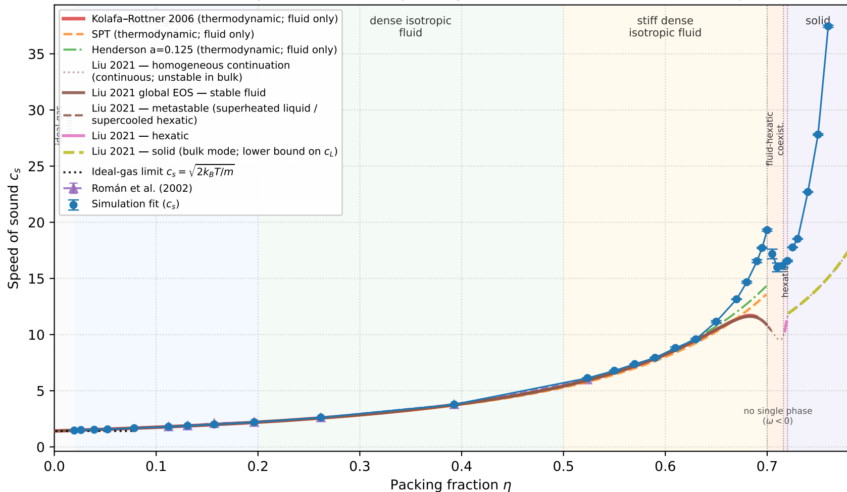
Hard disks: speed of sound vs packing fraction (r25, fixed core, 7200 traj)
